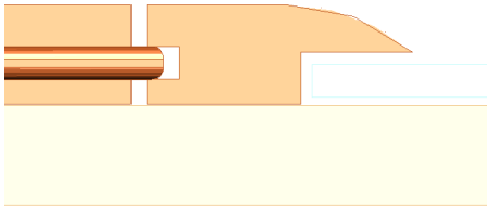
Fig. 9b Carpet reducer - section
