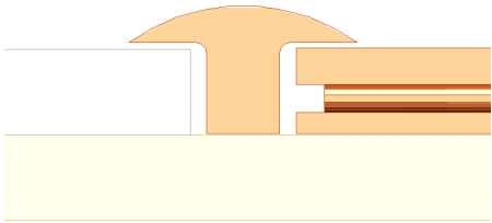
Fig. 8b T-cap reducer - section
